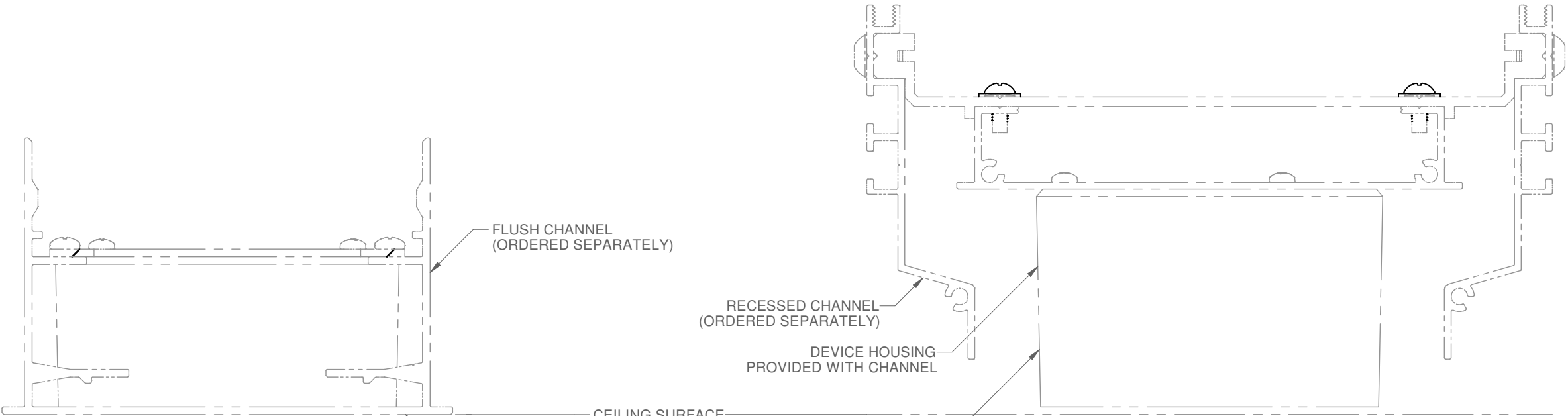
FLUSH CHANNEL END VIEW
