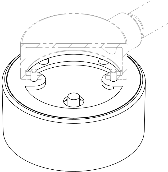
ISOMETRIC VIEW 20MM CONDUIT JUNCTION BOX
